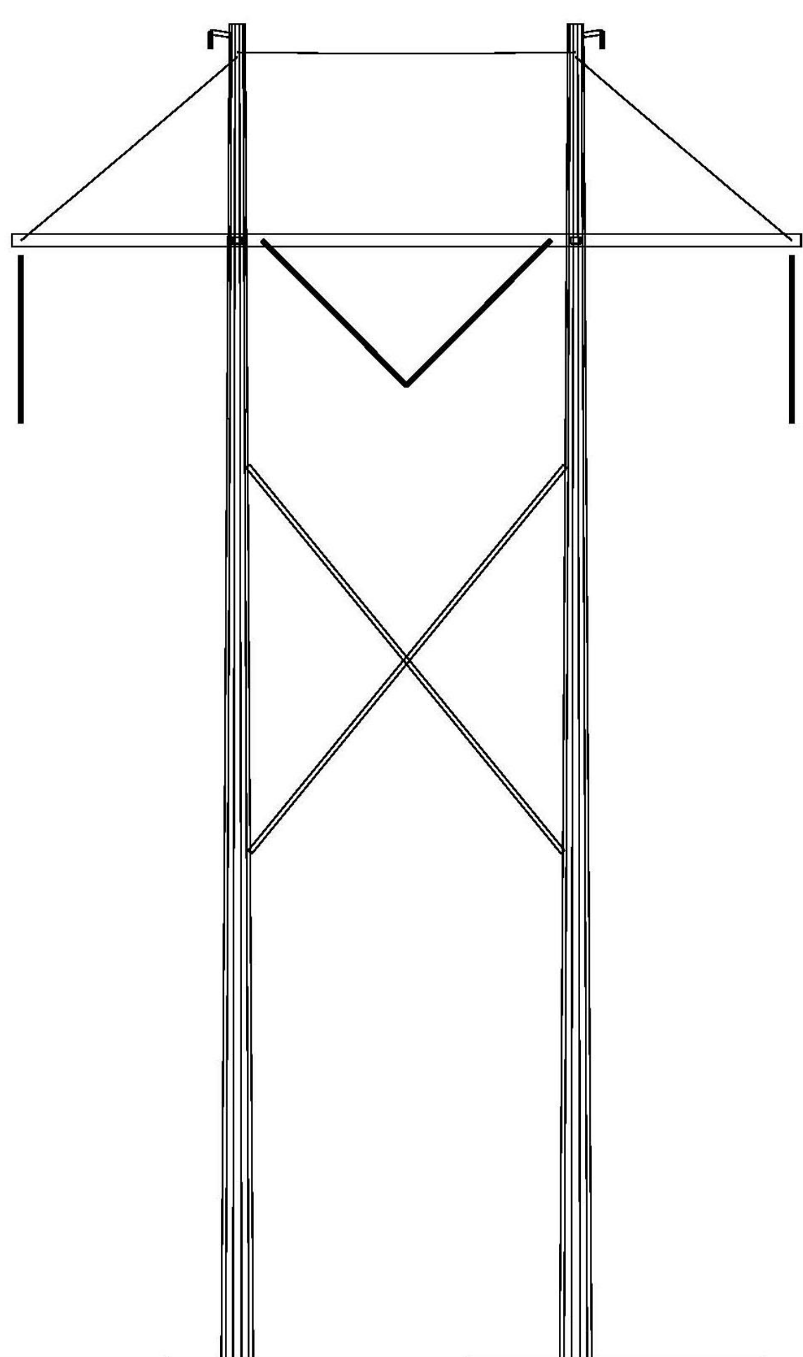
230 kV Single Circuit Steel H Frame 70' Height 120' Right-of-way
