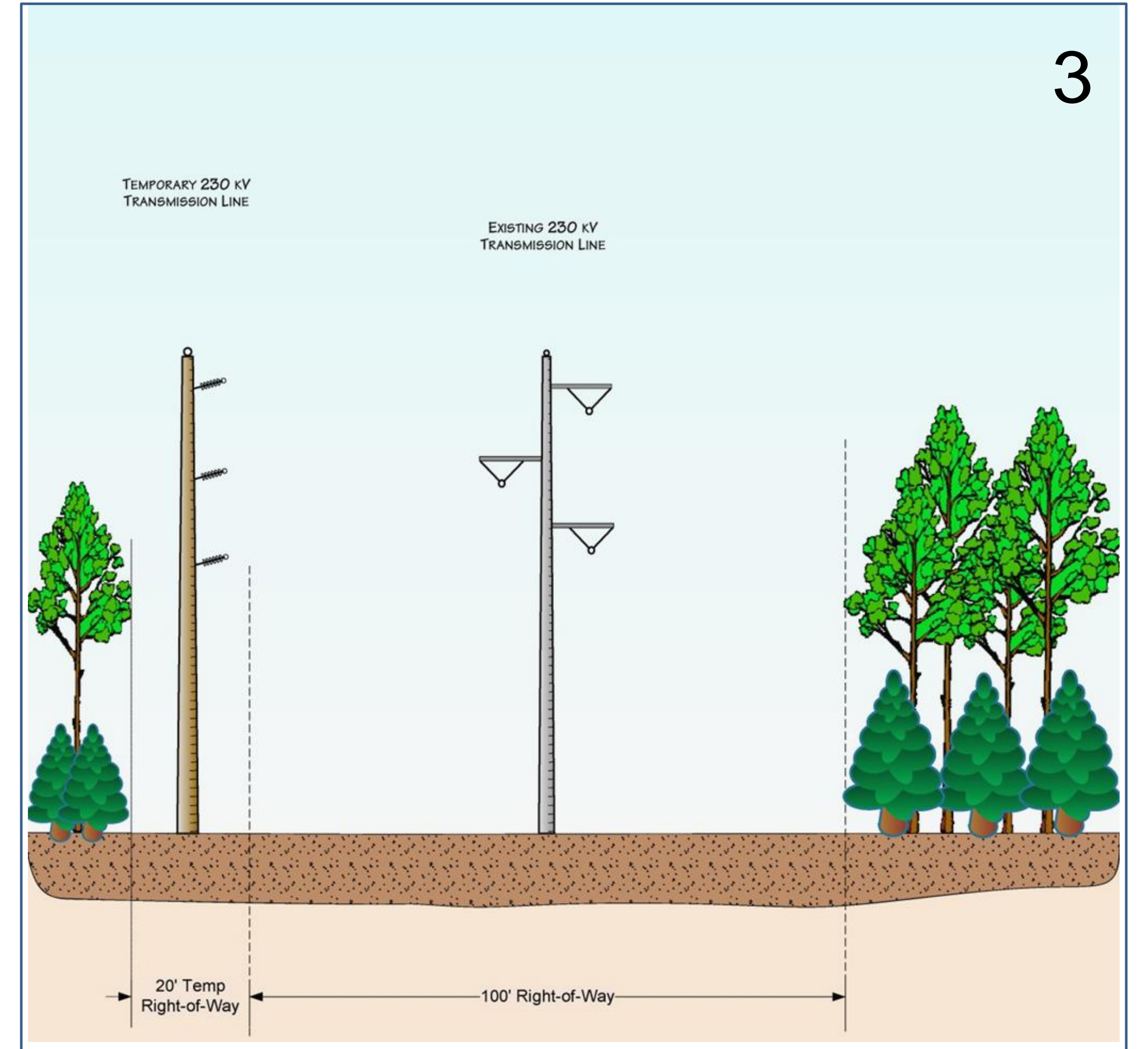
Erect and energize new, temporary 230 kV transmission line adjacent to existing line
