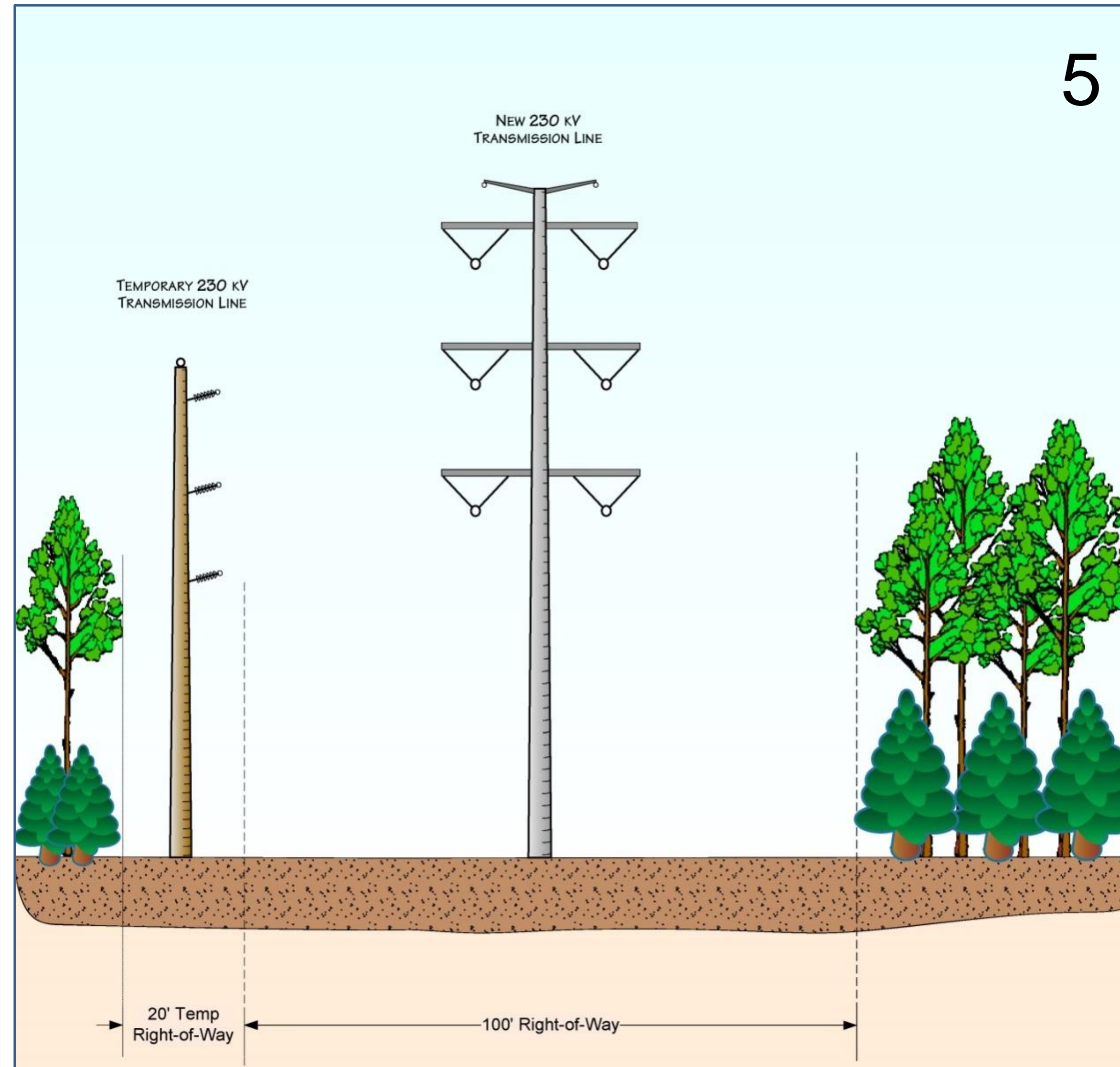
Build new double circuit 230 kV transmission line and energize
