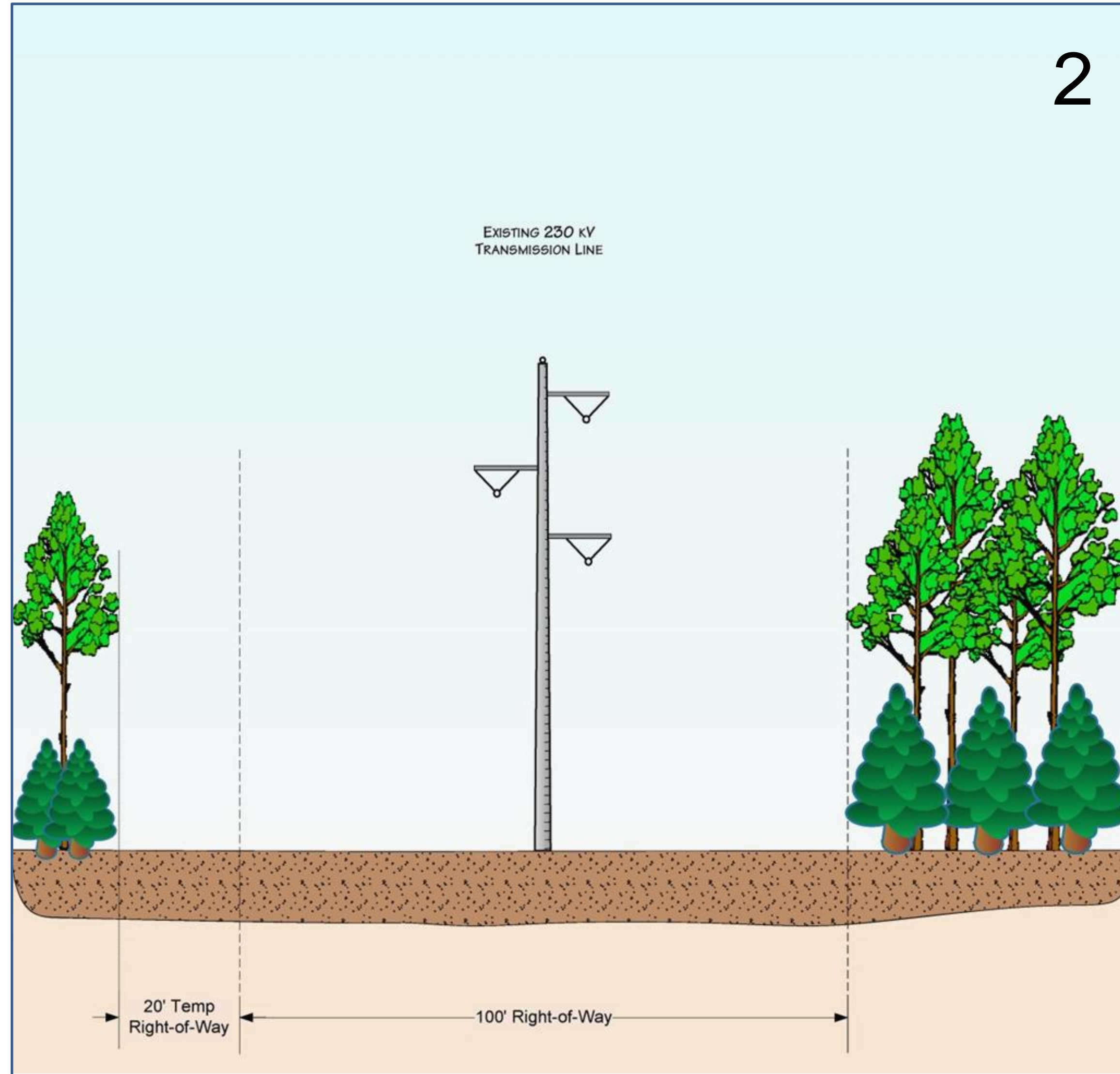
Clear 20 feet of temporary ROW adjacent to existing ROW
