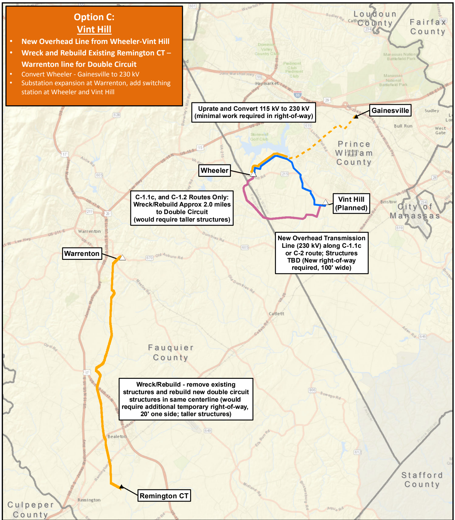
Figure 1-3 Option C Remington - Warrenton 230 kV Double Circuit Line Vint Hill - Wheeler and Wheeler - Gainesville 230 kV Transmission Lines Fauquier and Prince William Counties
