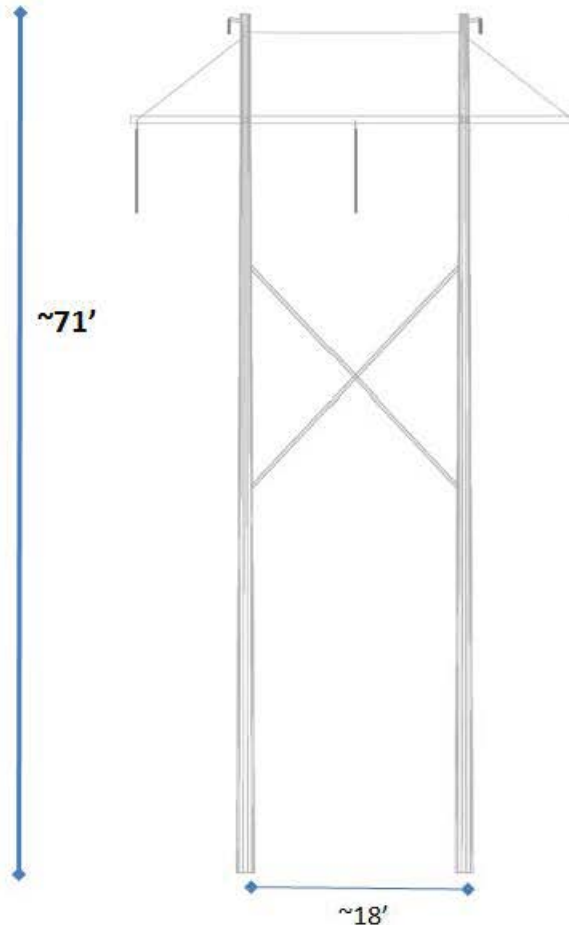
H-Frame Structure
