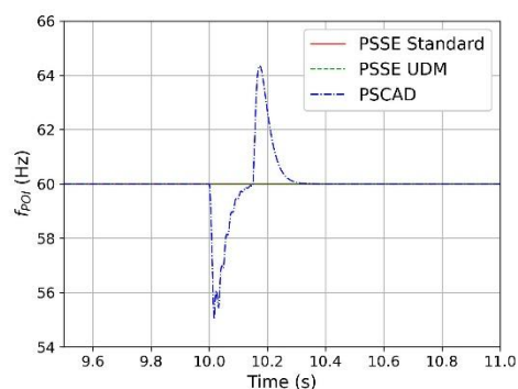
(a) Frequency at the POI
