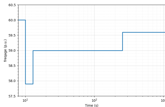
Figure 4. Frequency profile with data values at the POI for (a) HFRT test and (b) LFRT test
