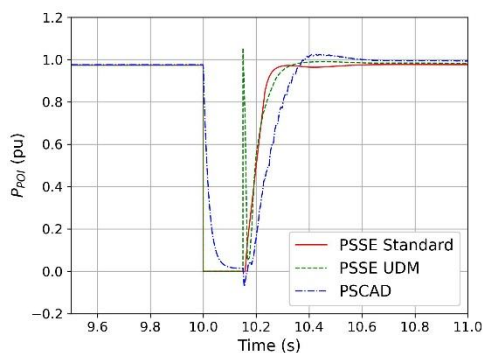
(c) Active power at the POI
