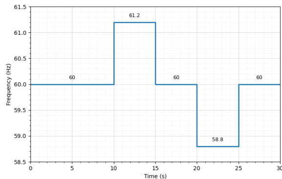
Figure 1. Frequency profile with data values at the POI for the frequency step tests
