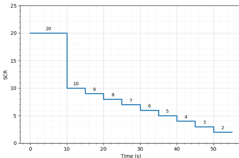
Figure 5. Short circuit ratio profile with data values of the grid for SCR tests
