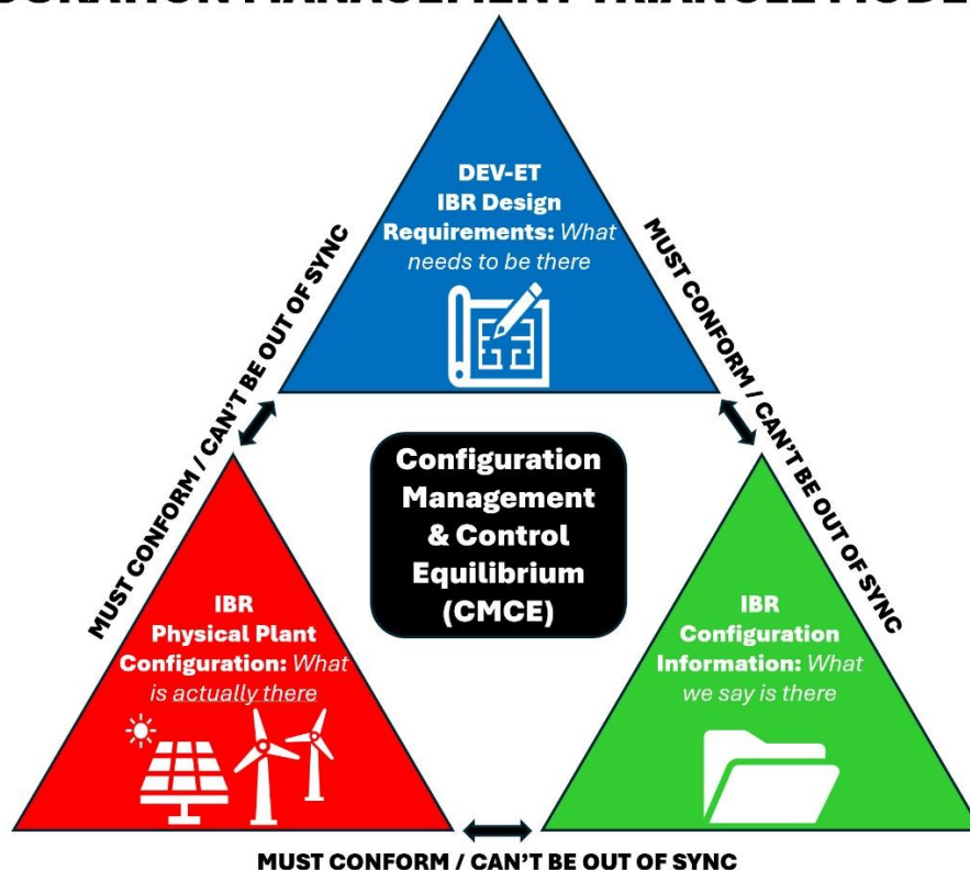
Figure 17. CMTM Model
