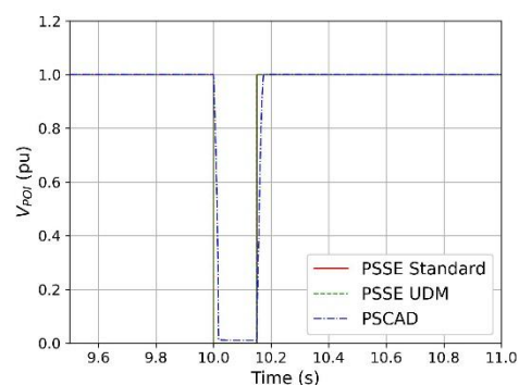
(b) Voltage at the POI
